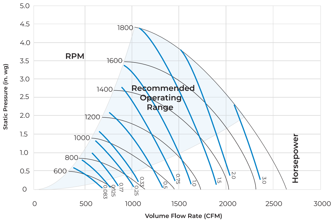
BBH HORIZONTAL / BBV VERTICAL FAN CURVES - SIZE 012
