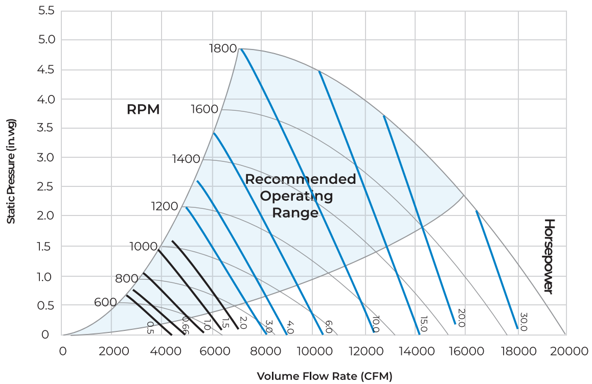
BBH HORIZONTAL / BBV VERTICAL FAN CURVES - SIZE 050
