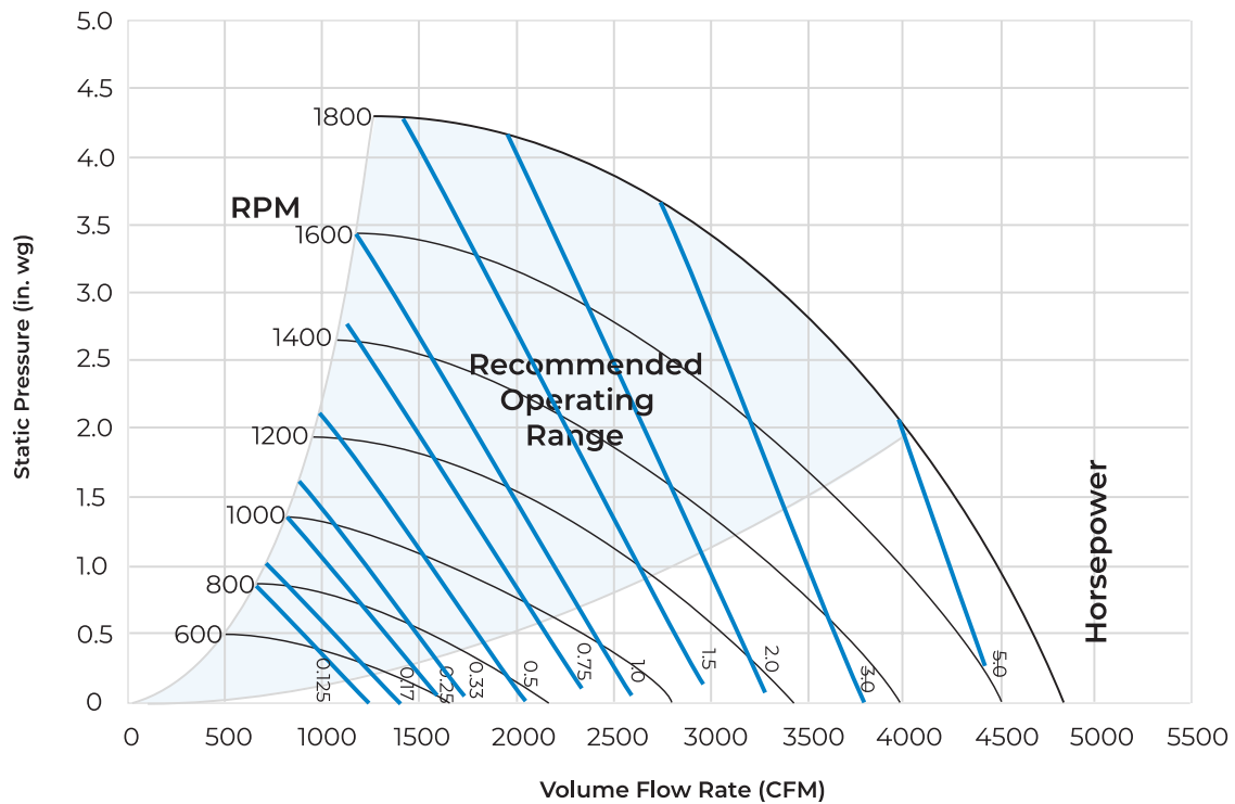
BBH HORIZONTAL / BBV VERTICAL FAN CURVES - SIZE 016
