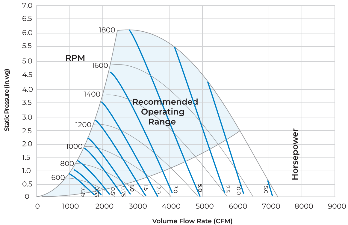
BBH HORIZONTAL / BBV VERTICAL FAN CURVES - SIZE 030
