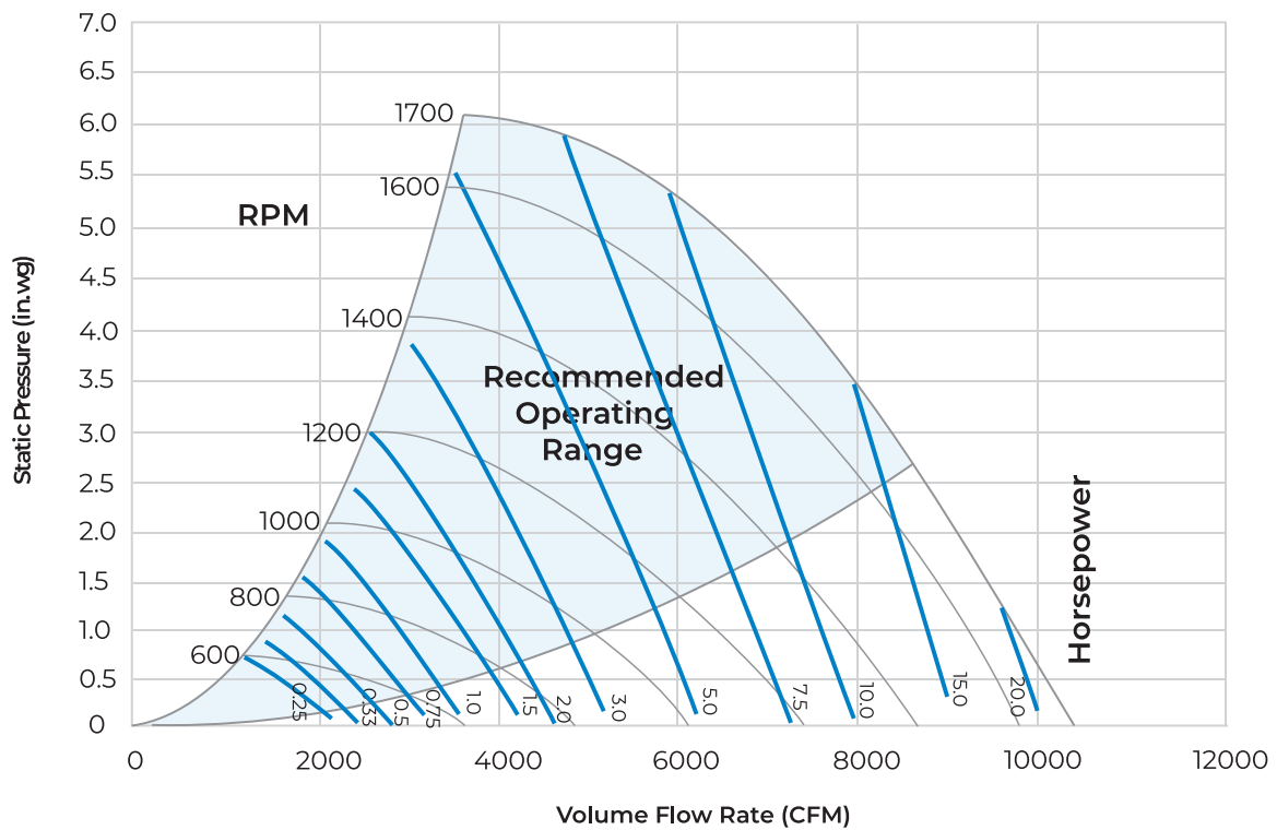
BBH HORIZONTAL / BBV VERTICAL FAN CURVES - SIZE 040
