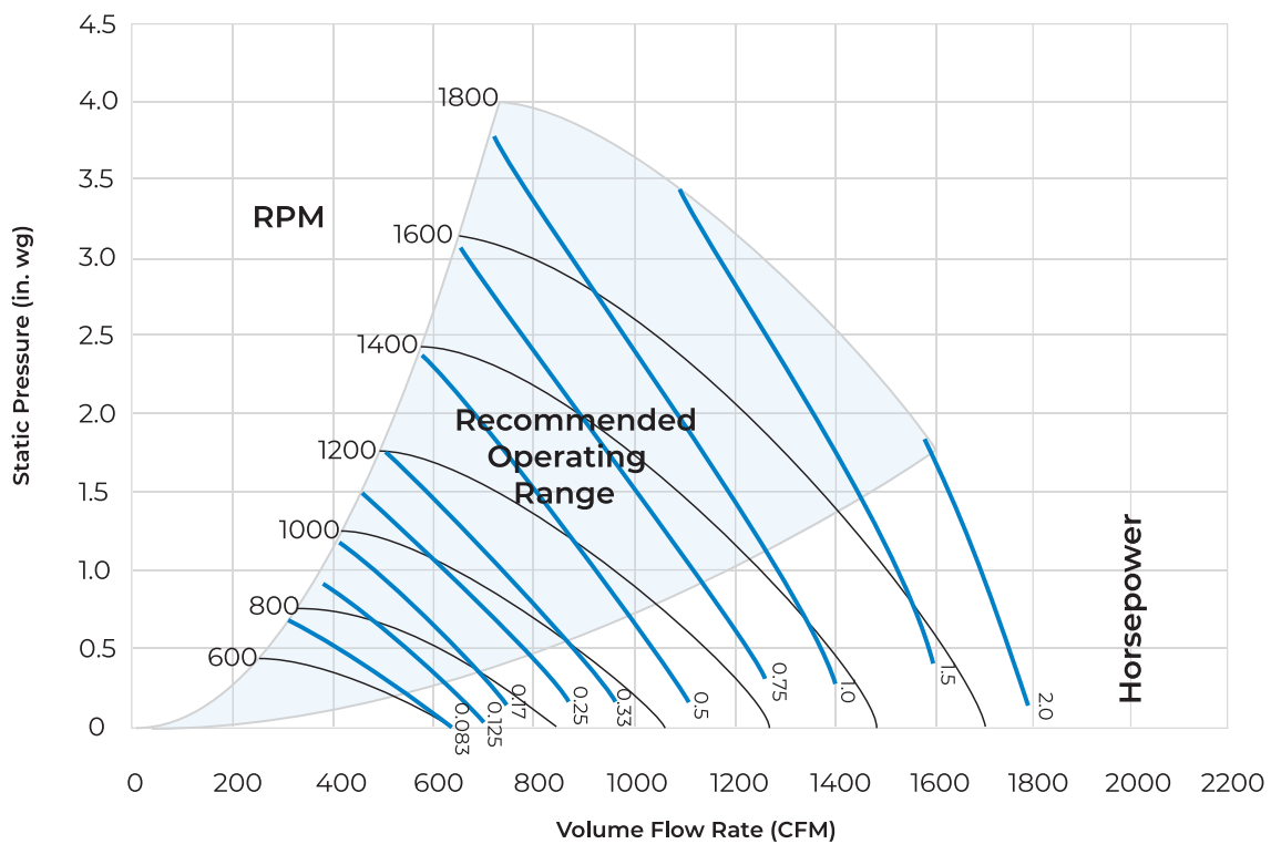
BBH HORIZONTAL / BBV VERTICAL FAN CURVES - SIZE 008
