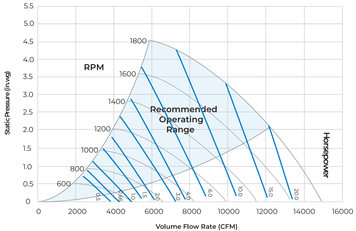
BBH HORIZONTAL / BBV VERTICAL FAN CURVES - SIZE 060
